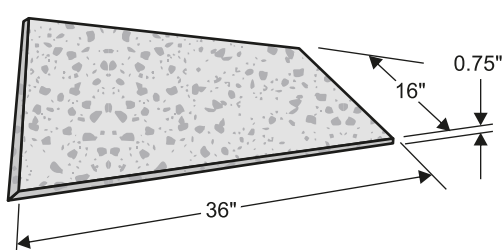
16" x 36" Standard Precast Slab
