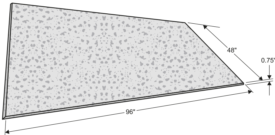
4' x 8' Standard Precast Slab
